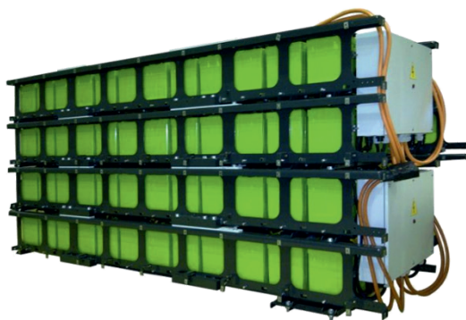
Pic. 3. Lithium-Iron Phosphate Battery
